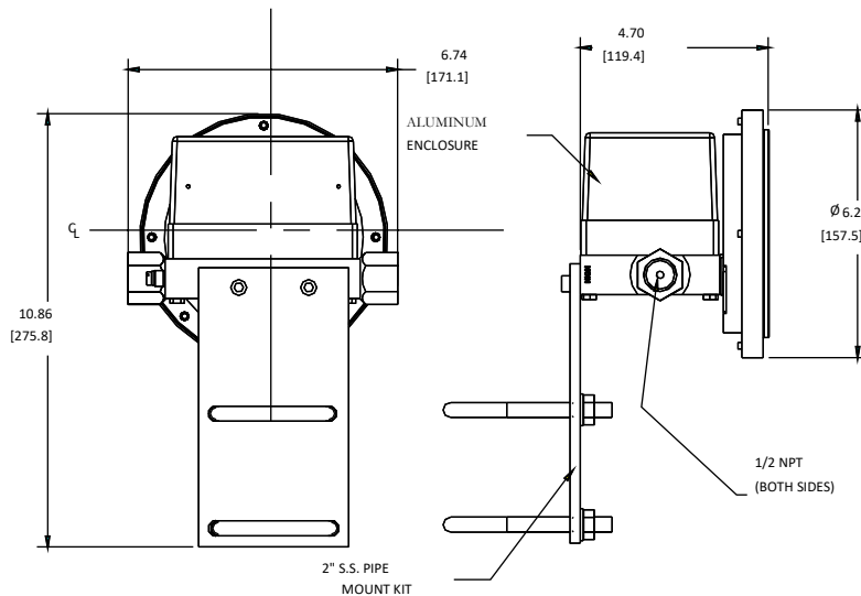
Figure 5 Typical SS 2" Pipe Mounting
