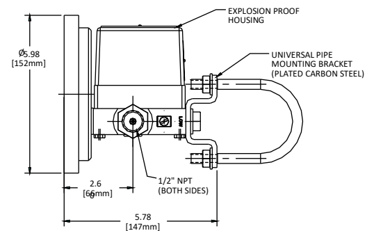
Figure 6 Typical CARBON Steel 2" Pipe Mounting
