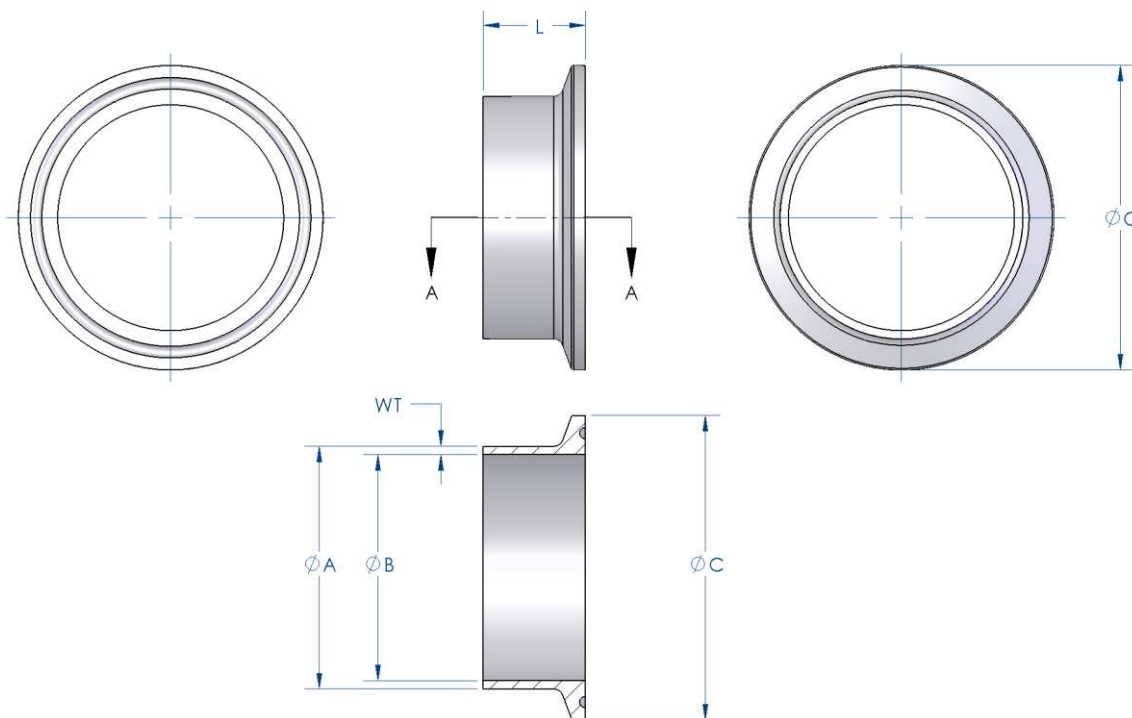
FERRULES - SCHEDULE 40
