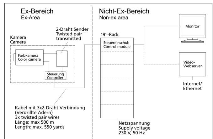
Lumiglas VISULEX K 06-Ex camera with fixed lens
